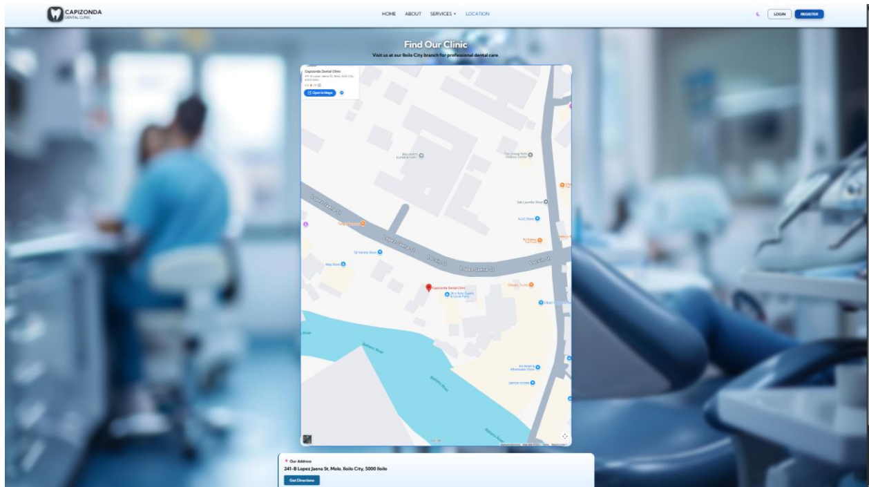
Figure 4.10 Location Page
