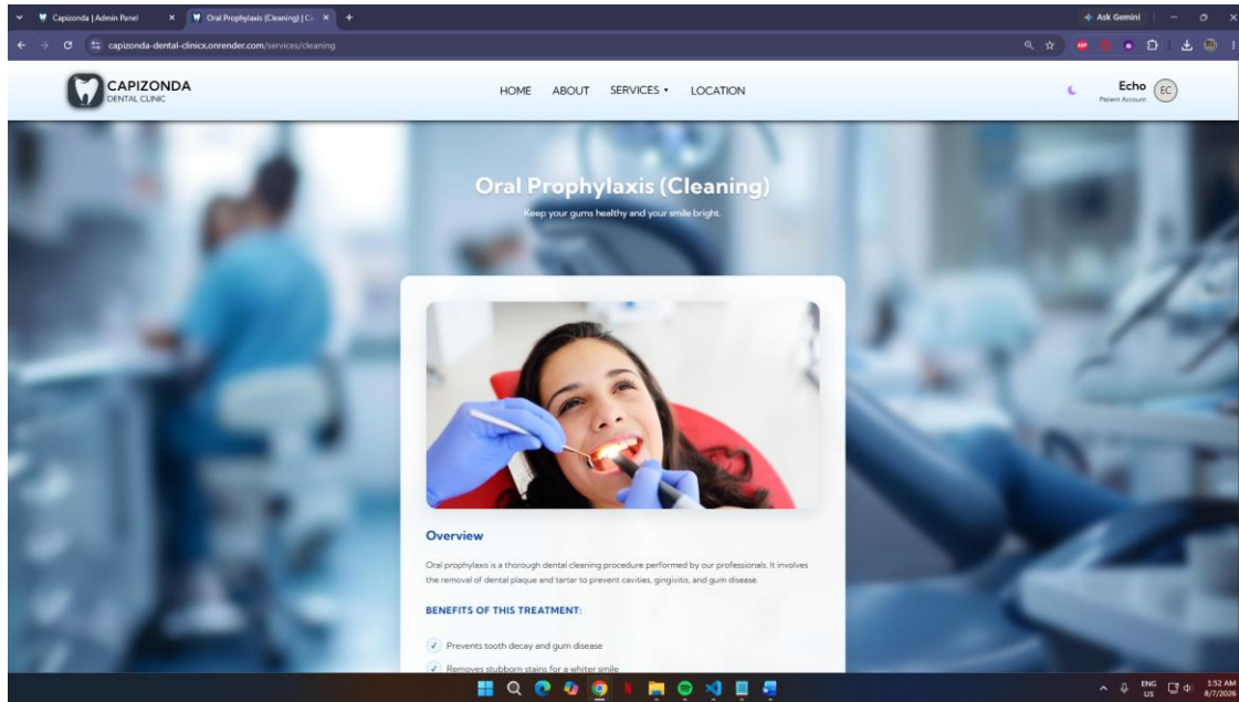
Figure 4.9 Service Page
