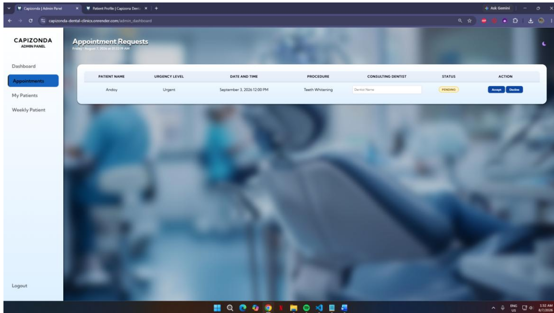
Figure 4.7 Appointment Module
