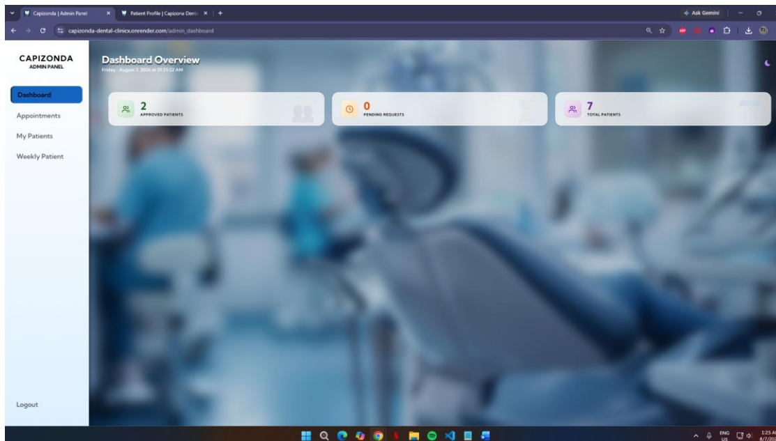
Figure 4.6 Admin Dashboard
